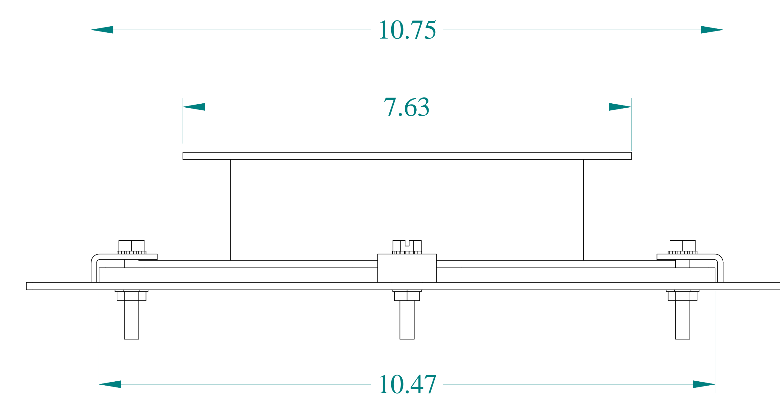
BOTTOM VIEW
