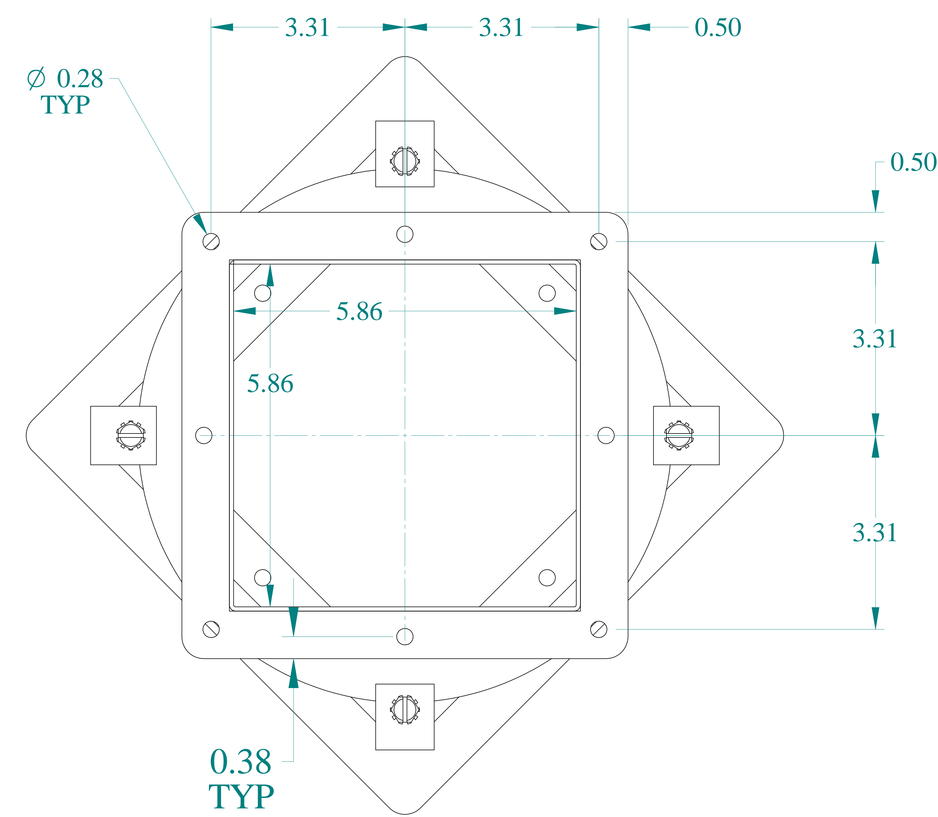
FRONT VIEW
