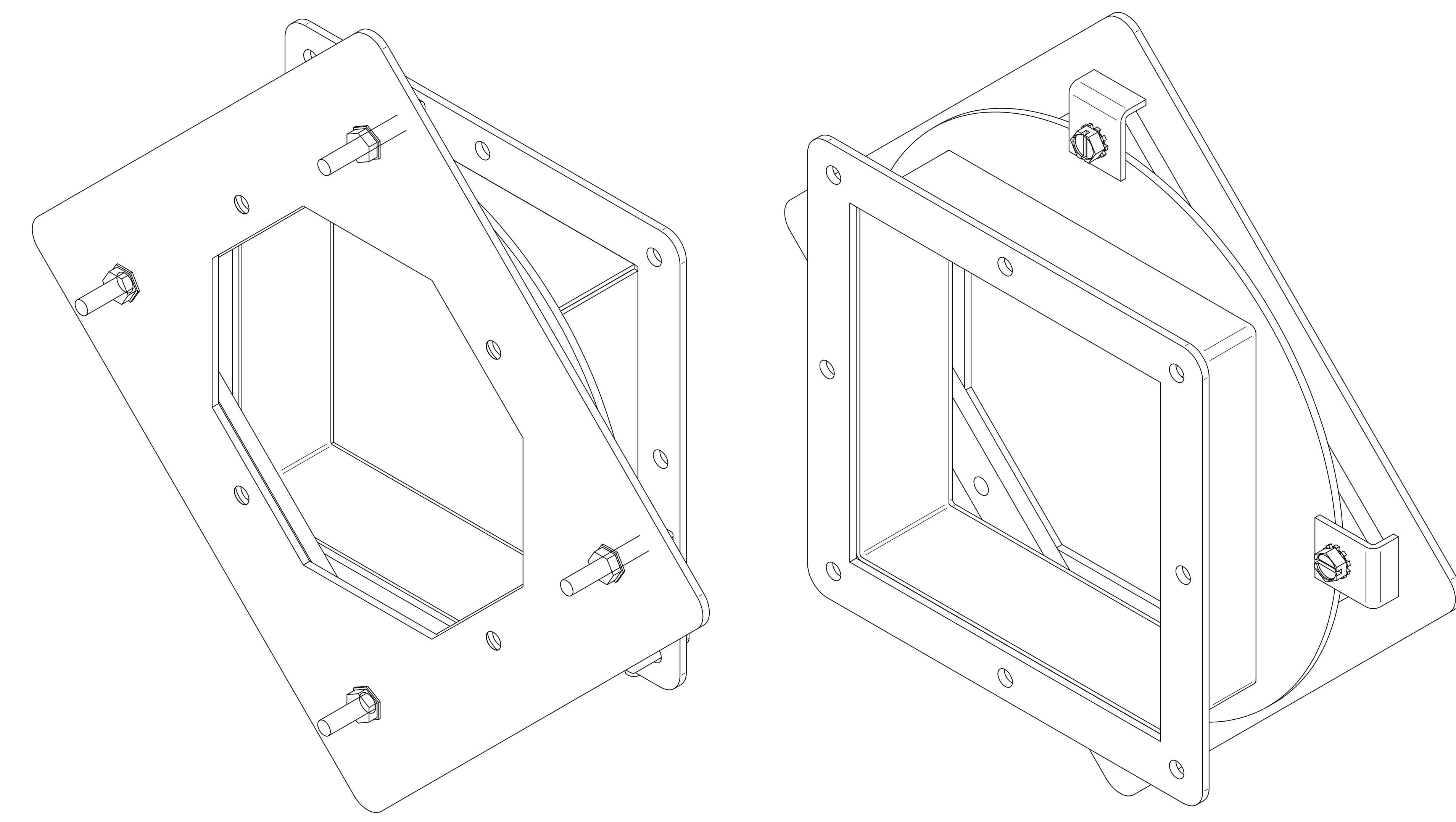
ISOMETRIC VIEWS
