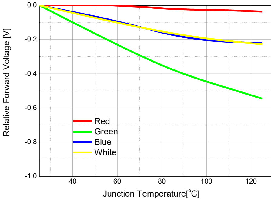
Junction Temperature vs. Forward Voltage at IF=1000mA
