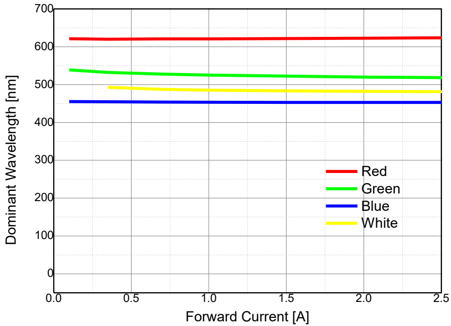
Forward Current vs Dominant Wavelength, T_j=25^\circ\text{C}
