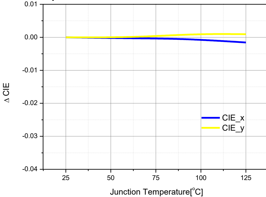
Junction Temperature vs. White ΔCIE at IF=1000mA
