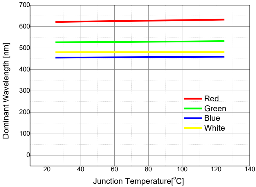
Junction Temperature vs. Dominant Wavelength at IF=1000mA
