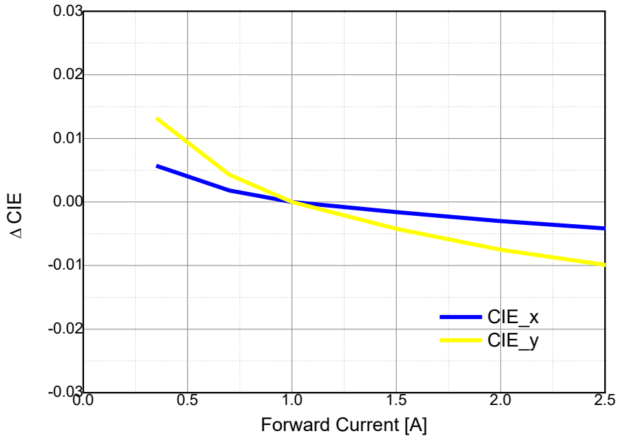
Forward Current vs \Delta CIE, T_j=25^\circ\text{C} (White)
