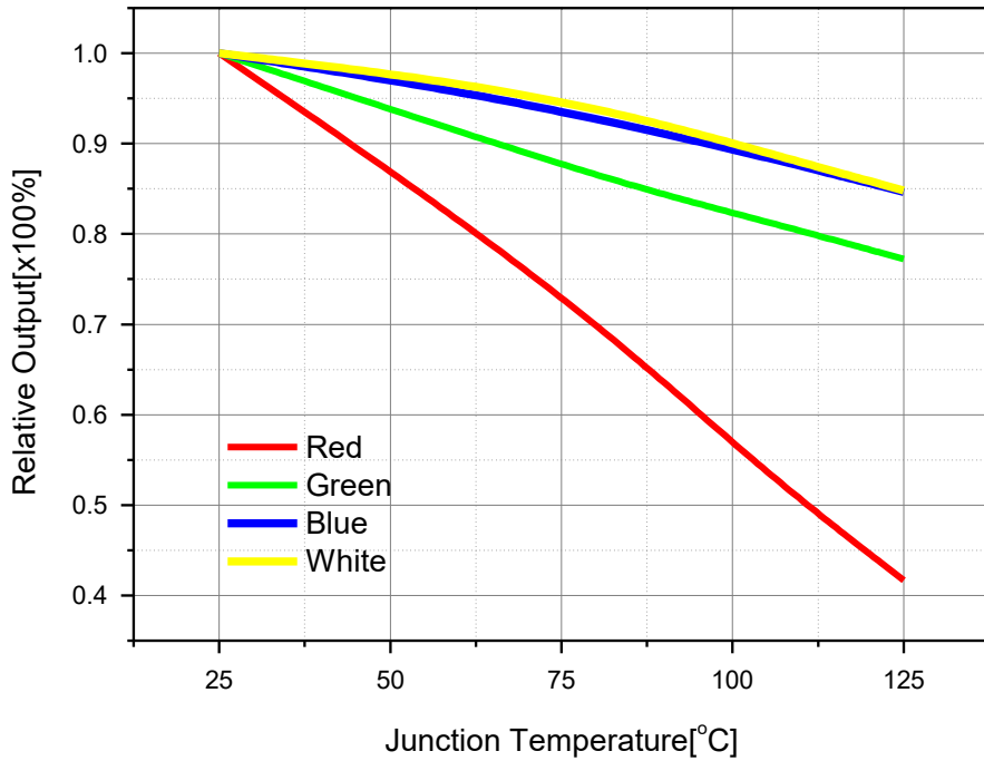
Junction Temperature vs. Relative Light Output at IF=1000mA
