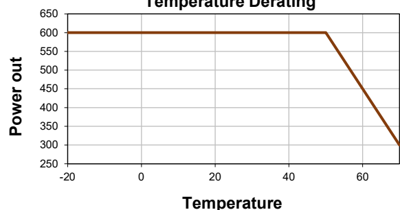
Temperature Derating
