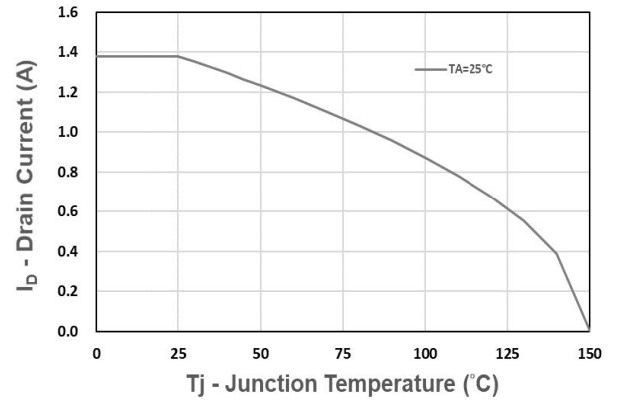
Figure 10. Drain Current
