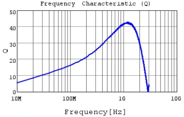
LQG15WZ23NJ02 Q
