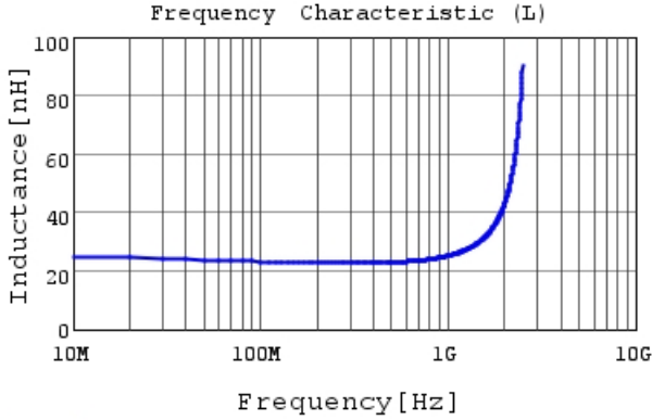
LQG15WZ23NJ02 L
