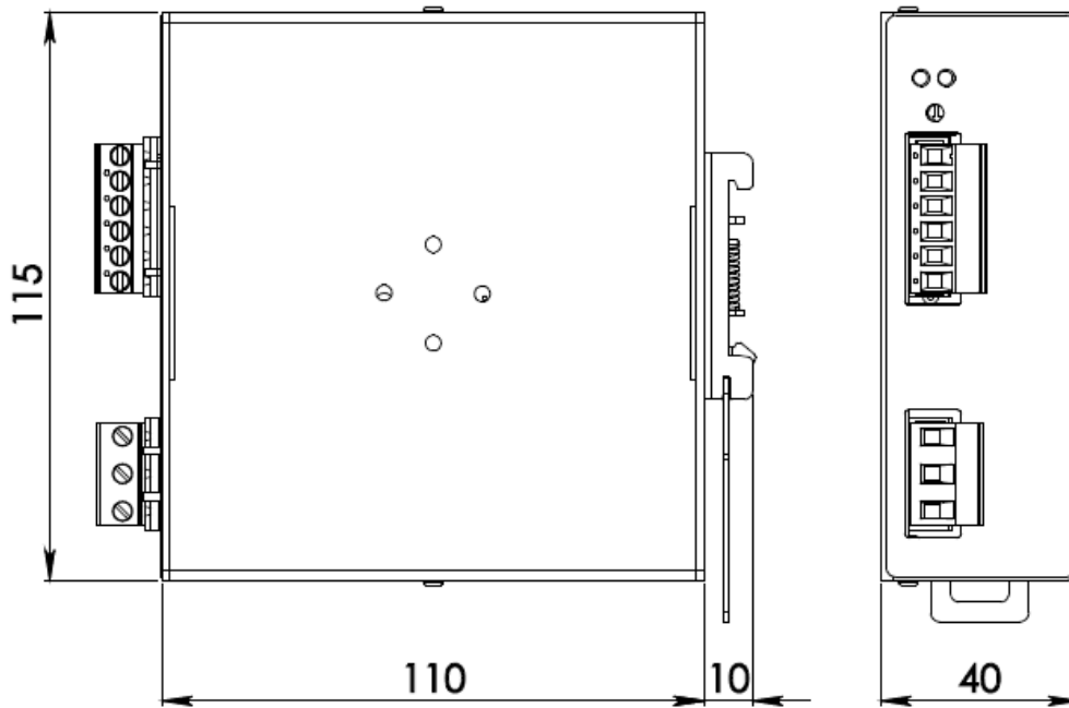
Figure 1. Mechanical Drawing
