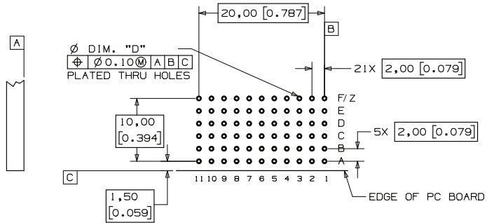
Recommended Hole Pattern for UHM-S055CL3-5AP1-XXXXX and UHM-S055CR3-5AP1-XXXXX
