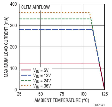
Derating, 3.3V _{OUT}
