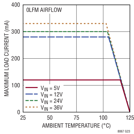
Derating, 2.5V _{OUT}
