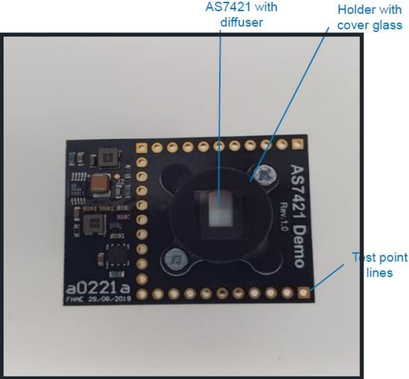
Fig. 2: Top view of the AS7421 sensor board with installed optomechanical parts
