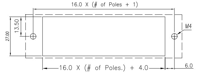
RECOMMENDED MOUNTING CUT-OUT
