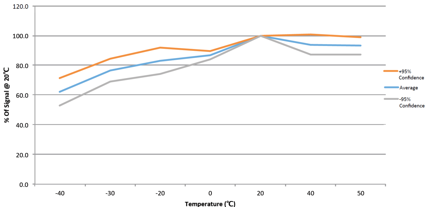
Output Temp. Coefficient data
