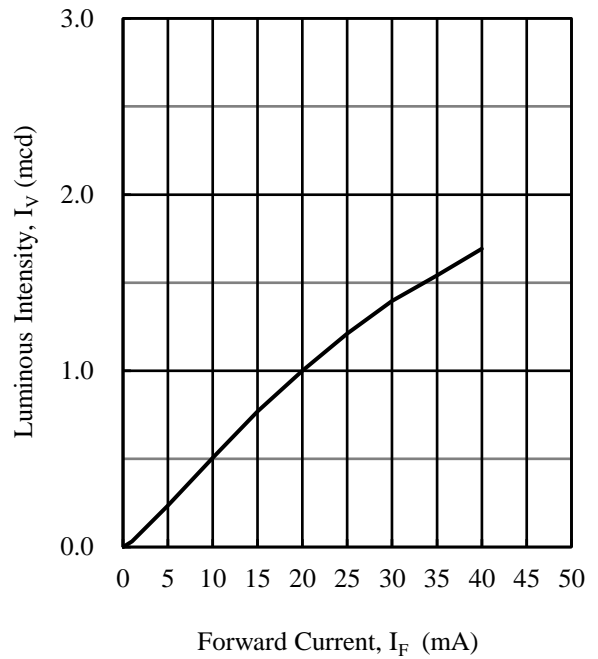
Figure 3. I_V vs. I_F
