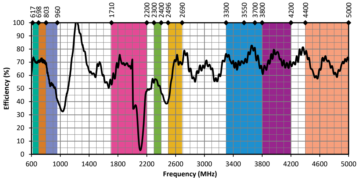
Figure 15. ANT-5GW-IPW1-NP Antenna Efficiency, Center of Ground Plane
