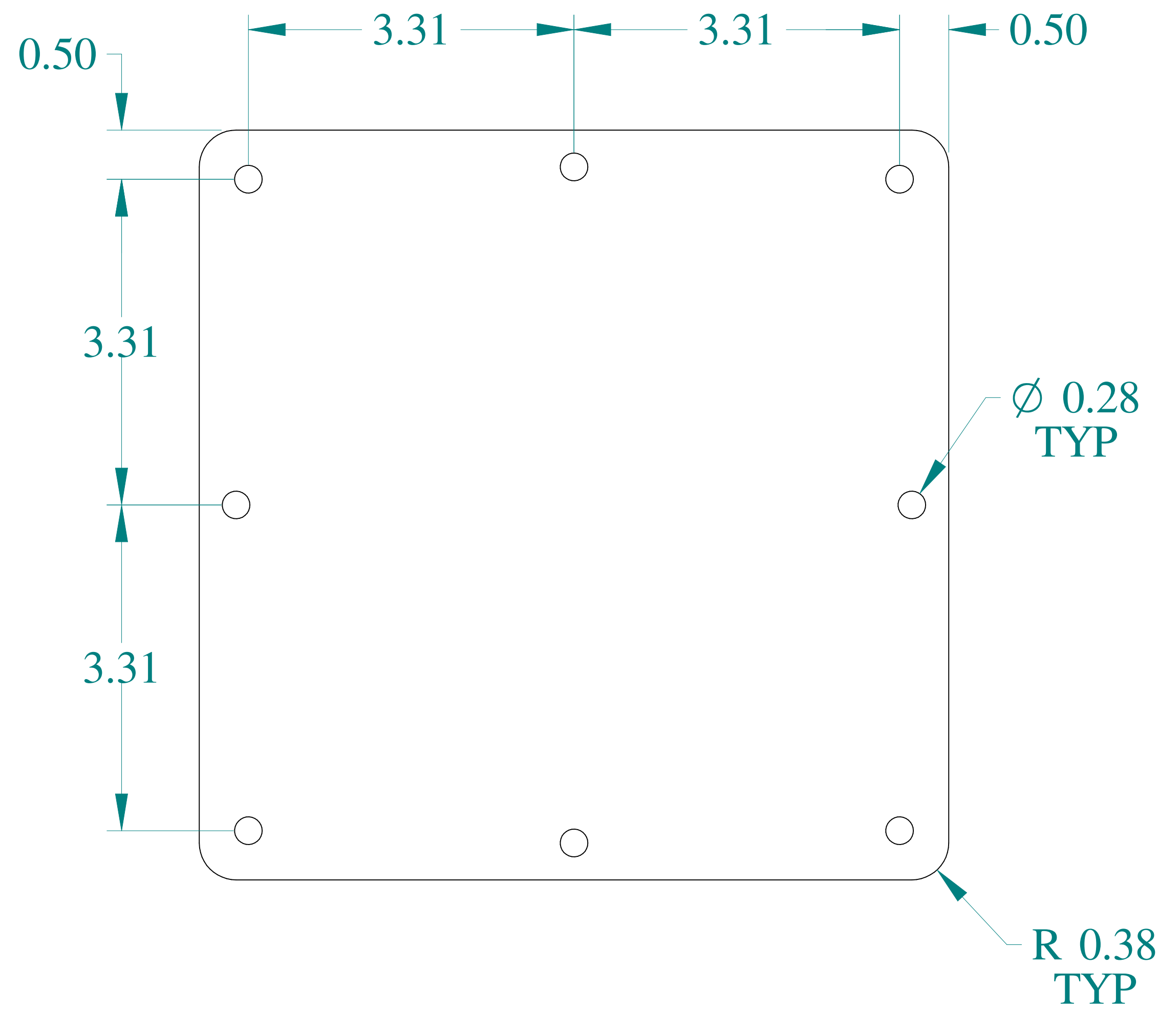
FRONT VIEW
