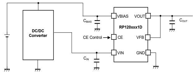
RP120 (Internal Fixed Type) Typical Application Circuit
