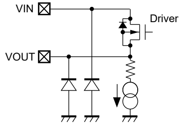
Internal equivalent circuit diagram of VIN and VOUT pin
