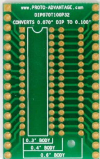
2D Top View (Pins Unassembled)
