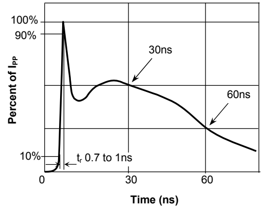
Figure 4. Pulse Waveform-ESD(IEC61000-4-2)
