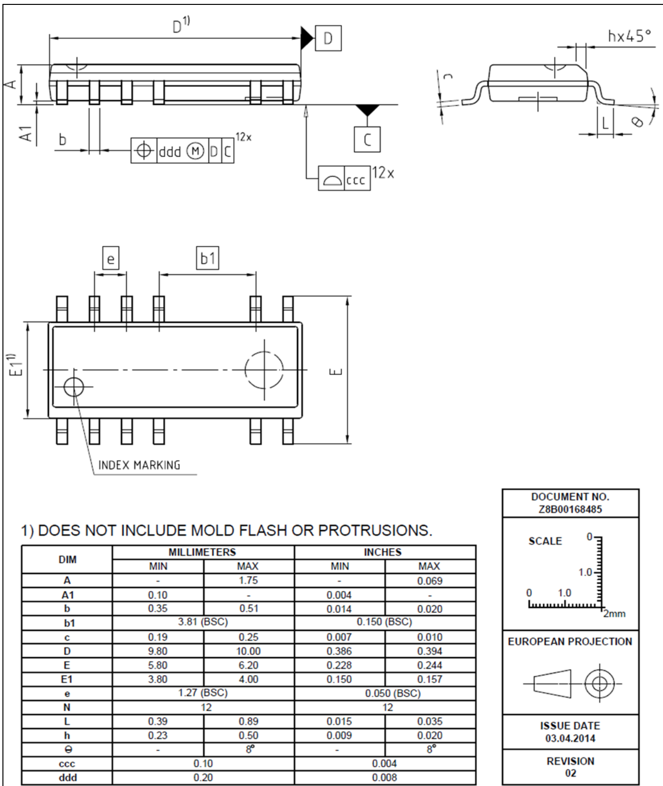
Figure 39 PG-DSO-12
