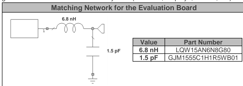
Figure 5 – Matching network implemented in the evaluation Board.
