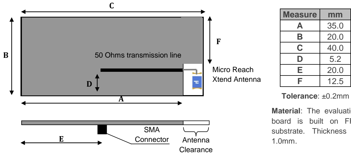
Figure 1 – EB_FR05-S1-N-0-110. Micro Reach Xtend™ Evaluation Board.
