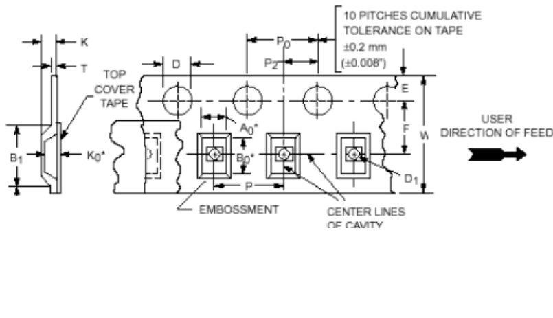
Figure 9 – Tape Dimensions and Tolerances.
