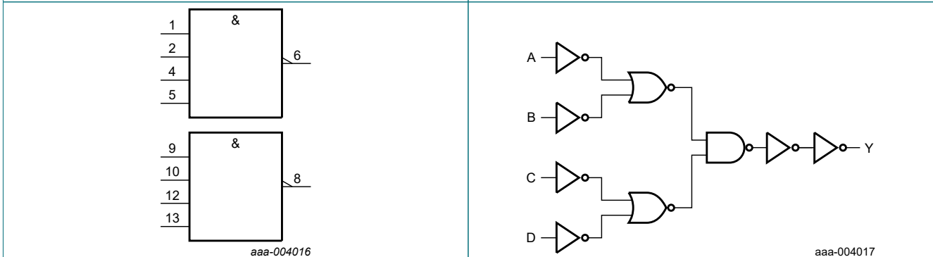
Fig. 3. IEC Logic symbol
