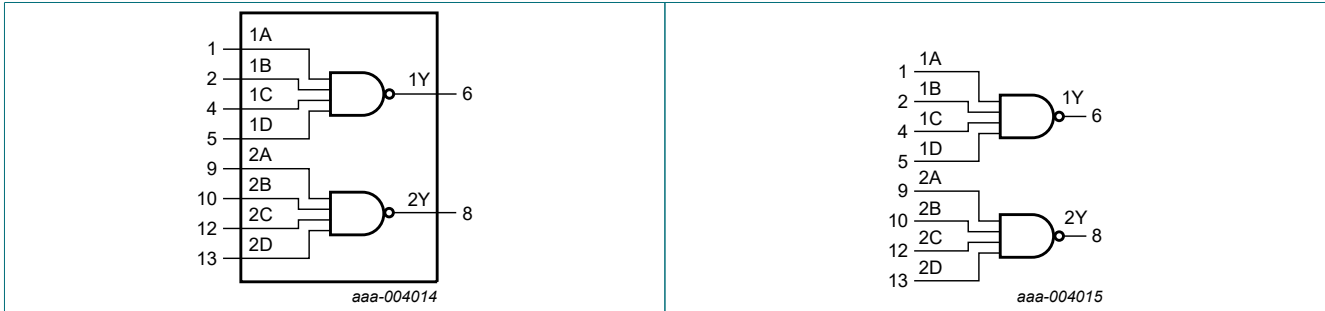
Fig. 1. Functional diagram
