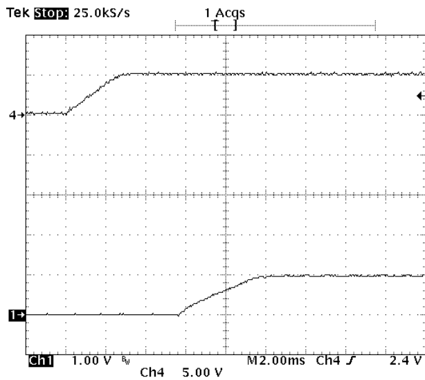
Fig-1.0V-4: Turn-on transient for V_{out}=1.0V with application of V_{in} at full rated load current (resistive) and 47\mu F \times 4 external capacitance at V_{in}=5.0V . Top trace: V_{in} (5V/div.) Bottom trace: output voltage (1V/div.) Time scale: 2ms/div.
