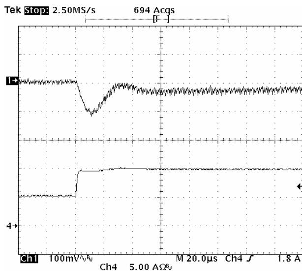
Fig-1.0V-6: Output voltage response for V_{out}=1.0V to positive load current step-change from 5A to 10A with slew rate of 5A/\mu s at V_{in}=5.0V . C_o=47\mu F \times 4 ceramic + 1\mu F ceramic. Top trace: output voltage (100mV/div.) Bottom trace: load current (5A/div.) Time scale: 20μs/div.
