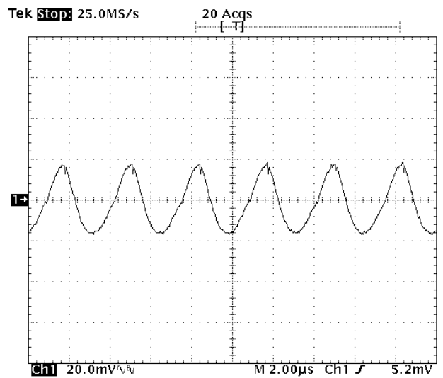
Fig-1.0V-5: Output voltage ripple (20mV/div.) for V_{out}=1.0V at full rated load current into a resistive load with external capacitance 47\mu F \times 4 ceramic + 1\mu F ceramic at V_{in}=5.0V . Time scale: 2μs/div
