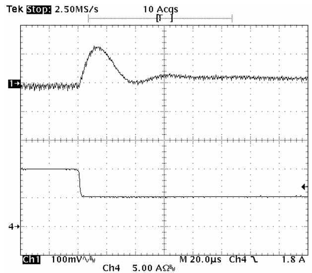
Fig-1.0V-7: Output voltage response for V_{out}=1.0V to positive load current step-change from 10A to 5A with slew rate of -5A/\mu s at V_{in}=5.0V . C_o=47\mu F \times 4 ceramic + 1\mu F ceramic. Top trace: output voltage (100mV/div.) Bottom trace: load current (5A/div.) Time scale: 20μs/div.
