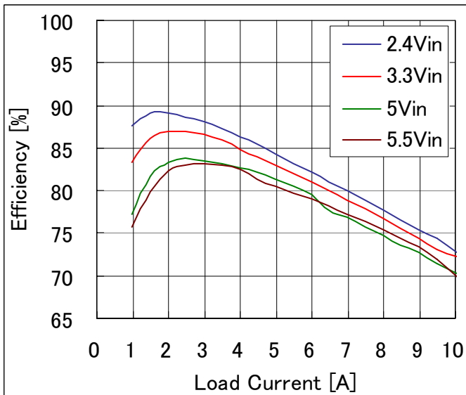
Fig-0.7255V-2: Efficiency vs. load current and input voltage for Vout=0.7525V. Airflow rate=200 LFM (1.0m/s) and Ta=25°C.
