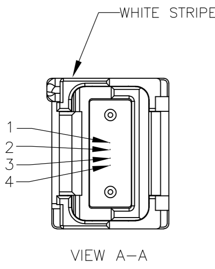
LIGHTRAY MPX CONNECTOR FIBER PATH
