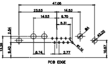
13W6 Male
