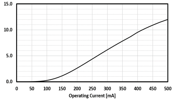
FIG. 2: SLED OUTPUT POWER VS CURRENT
