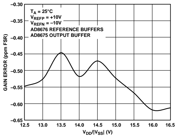
Figure 25. Gain Error vs. Supply Voltage, ±10 V Span
