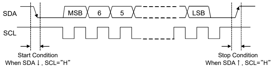
Figure 6. Command Interface
