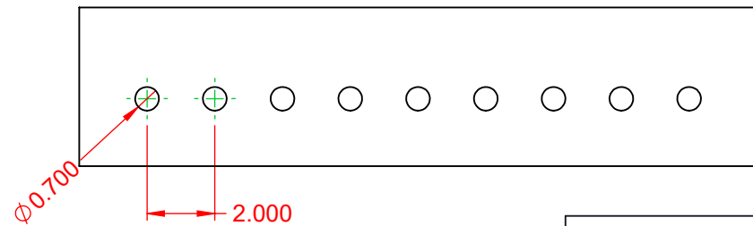
SUGGESTED PCB LAYOUT
