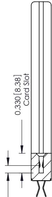
0.125 [3.18] Point of Contact — SECTION A-A
