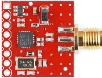
SparkFun Transceiver Breakout - nRF24L01+ with RP-SMA antenna (WRL-00705)
