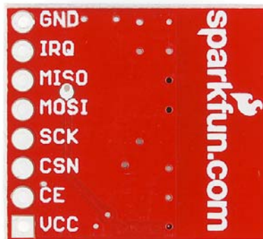
Broken out pins with labels
