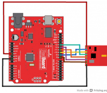
nRF24L01+ Circuit Assembly
