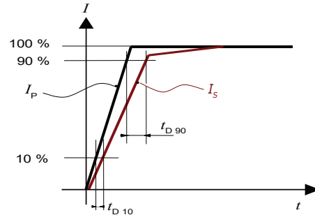
Figure 5: t_{D10} (delay time @ 10 %) and t_{D90} (delay time @ 90 %).
