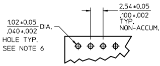
TYP. HOLE PATTERN FOR 1.57/.062 THK. PCB
