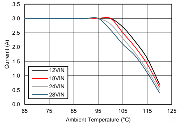
Figure 78. Derating Curve
