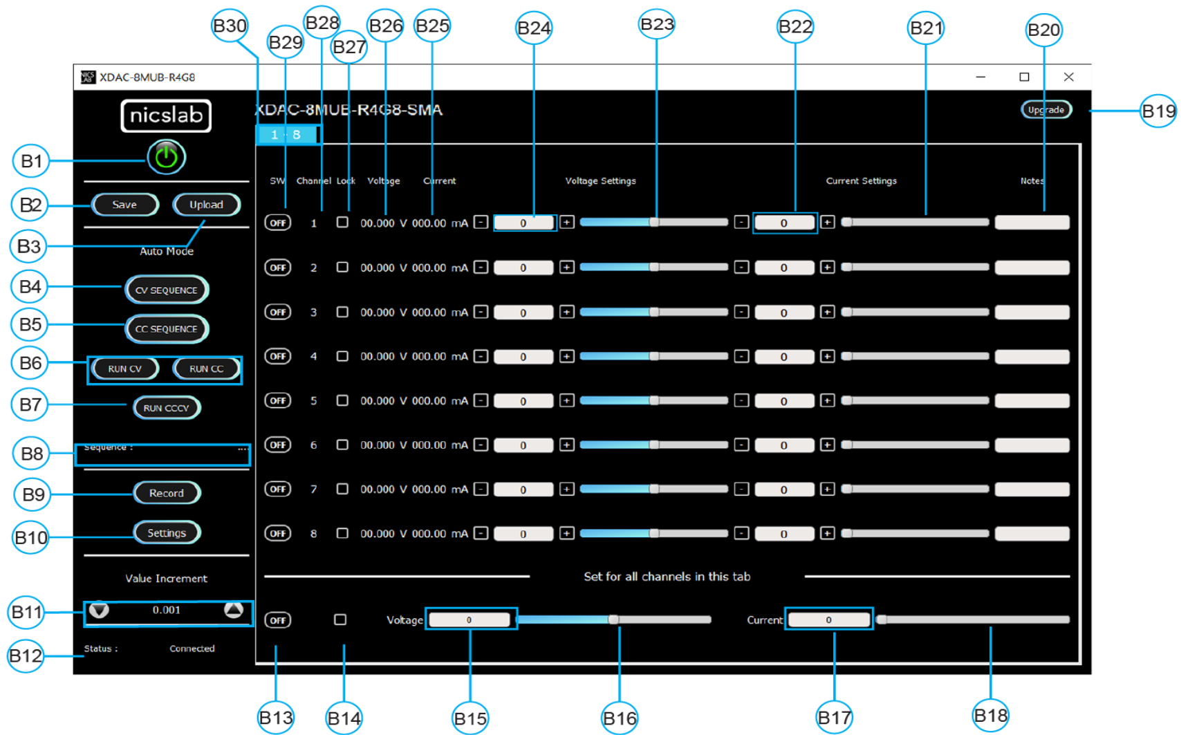
Figure 4. GUI
