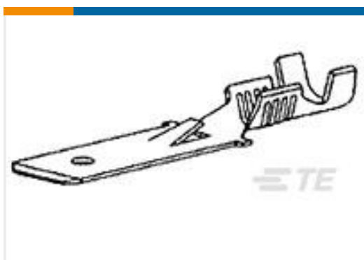
TE Part #160762-2 FF 110 TAB 0.5-1.5MM2 PTPBR
