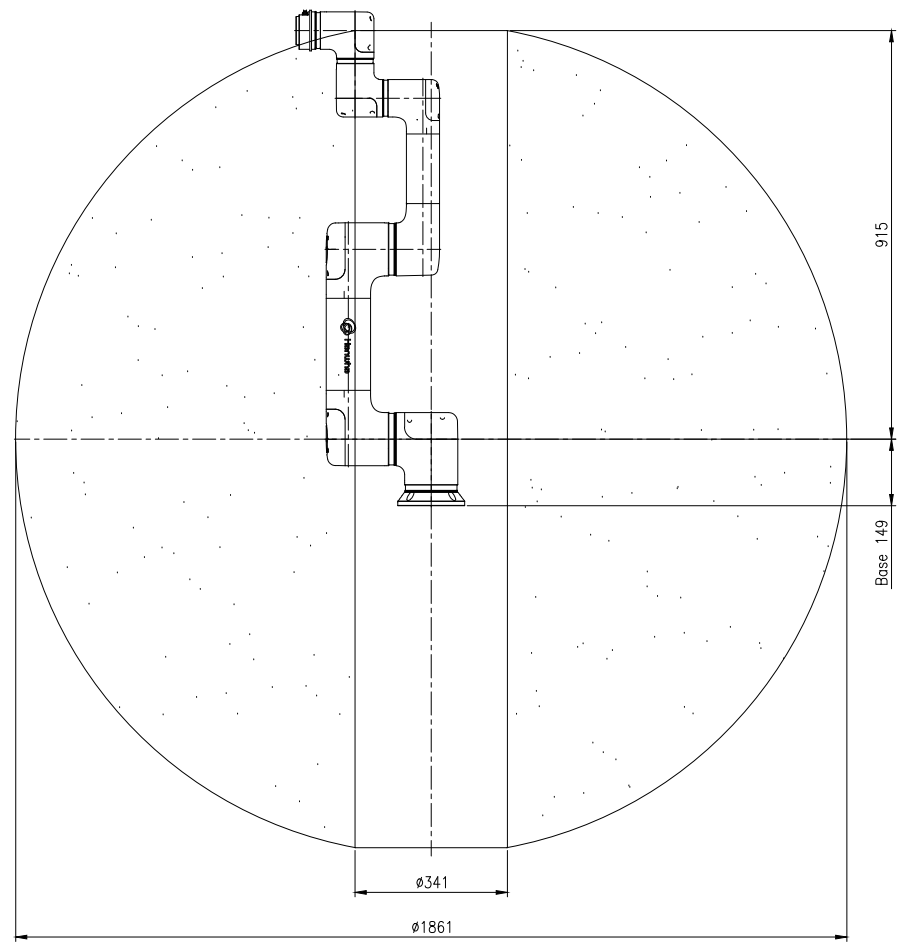
HCR-5A Working area, side view
