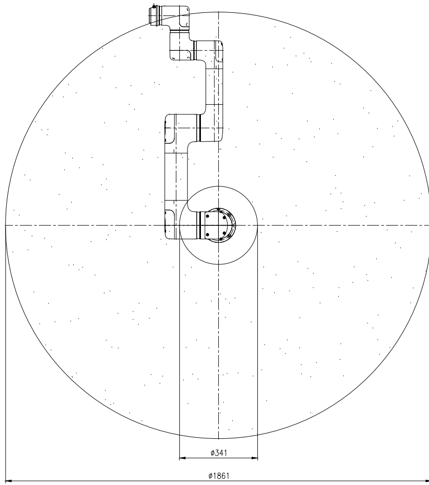
HCR-5A Working area, top view
