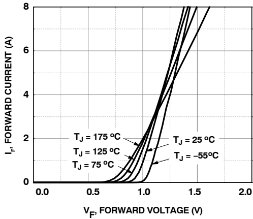
Figure 1. Forward Characteristics
