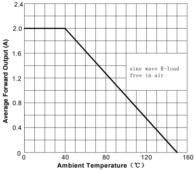
FIG1:Io-Ta Curve
