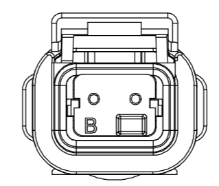
KEY-B CONFIGURATION ATMH04-2PB TPA COLOR: BLACK
