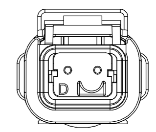
KEY-D CONFIGURATION ATMH04-2PD TPA COLOR: BROWN
