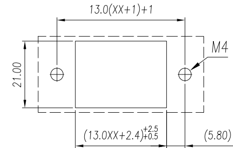
RECOMMENDED MOUNTING CUT-OUT
