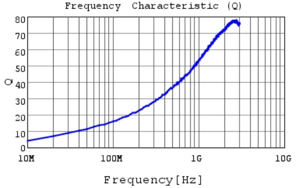
LQG15WH3N7B02 Q
