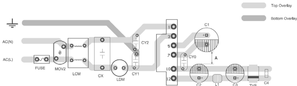
Recommended EMC circuit-PCB layout
