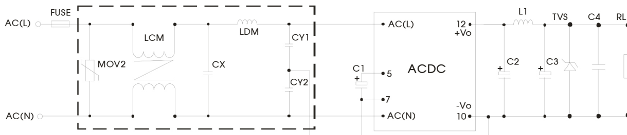
EMC application circuit with higher requirements
