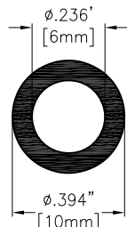
O-Ring ø6/2T, Black
