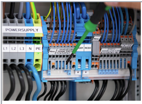
Tool-operated N-disconnect slide link
