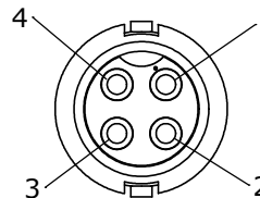
FACE VIEW 6382-4PG-5XX
