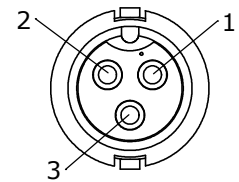
FACE VIEW 6382-3PG-5XX
