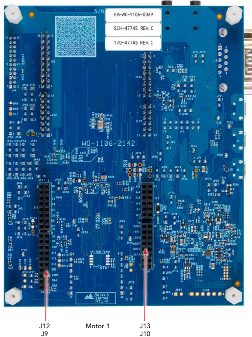
Figure 2: LPC5536-EVK Pin-Out
