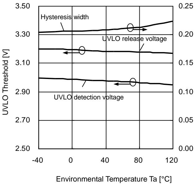
Figure 10. UVLO Threshold vs Environmental Temperature (UVLO Threshold)
