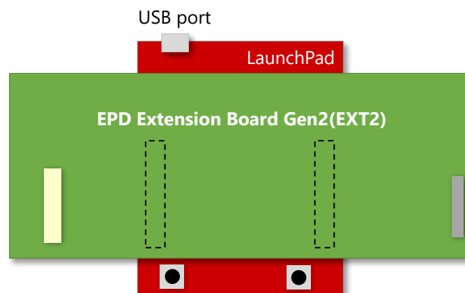
Figure 2-1 Stack EXT2 on LaunchPad
