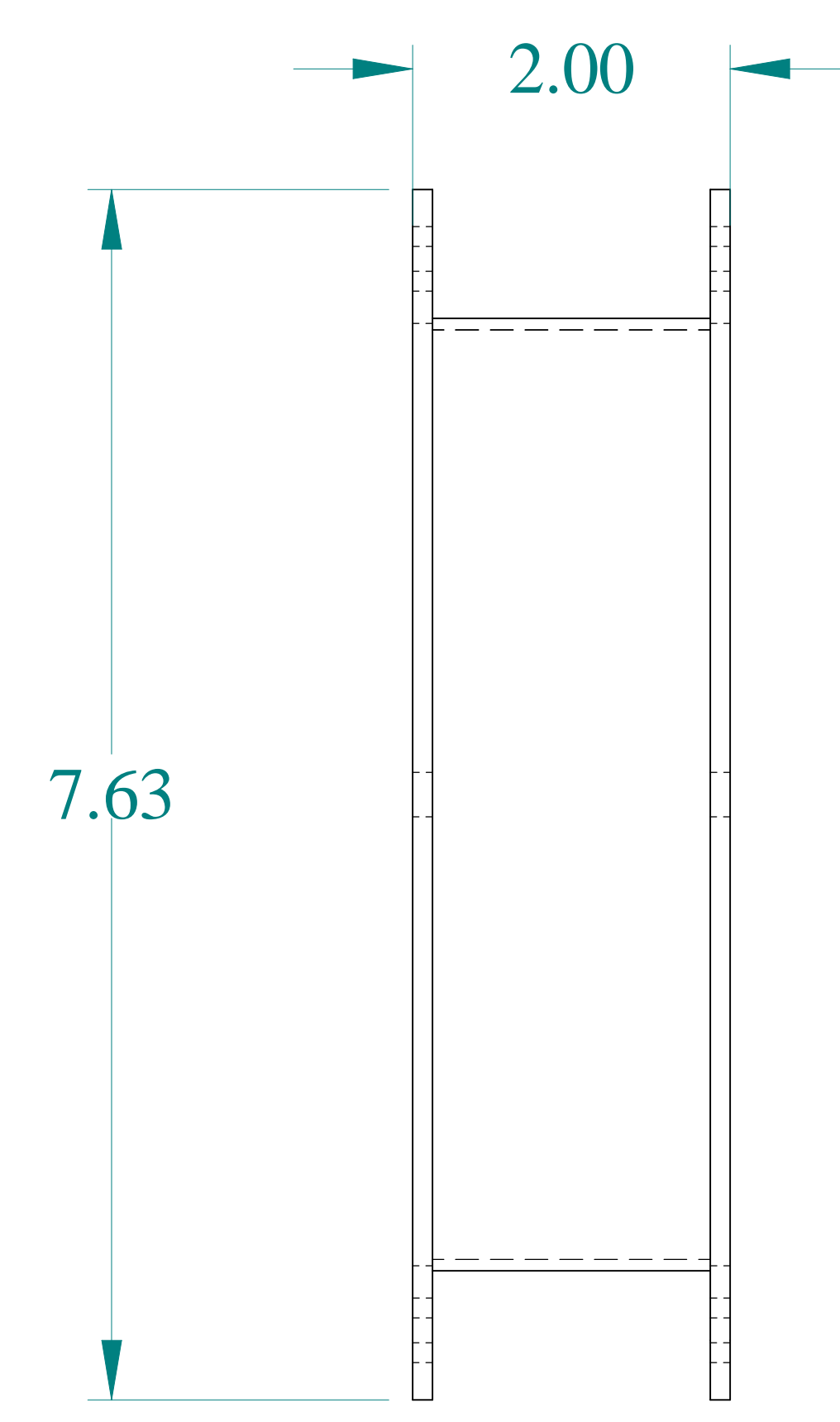
TOP VIEW
