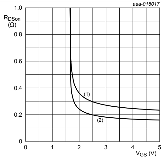
Fig. 10. Drain-source on-state resistance as a function of gate-source voltage; typical values I_D = 0.2\text{ A} (1) T_j = 150\text{ °C} (2) T_j = 25\text{ °C}
