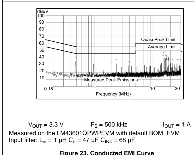
Figure 23. Conducted EMI Curve
