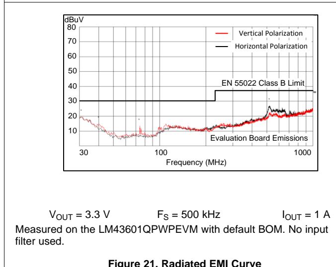
Figure 21. Radiated EMI Curve
