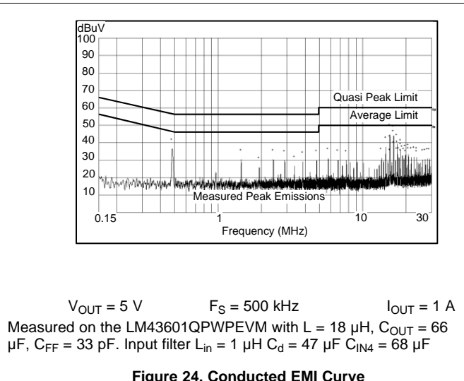
Figure 24. Conducted EMI Curve
